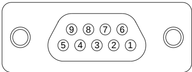
9-WAY 'D' PLUG FACE VIEW
