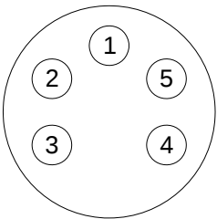
MCIL5F PIGTAIL FACE VIEW
